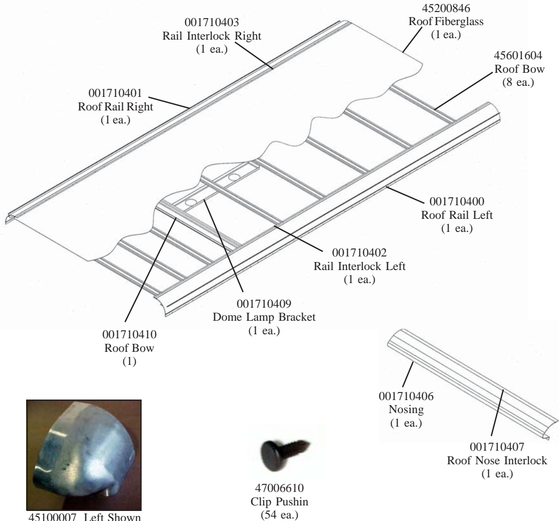
45100007 Left Shown 45100008 Right Opposite Front Roof Corner Casting (1 ea.)
