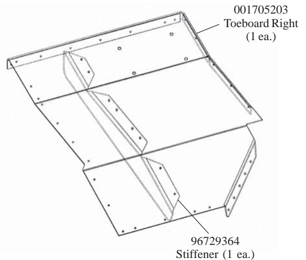
TOEBOARD ASSEMBLY RIGHT
